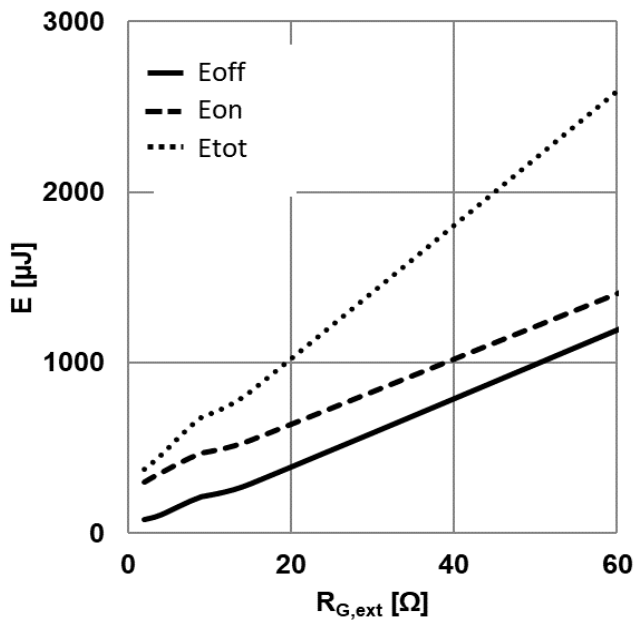
Figure 17 Typical switching energy losses as a function of gate resistance ( E = f(R_{G,ext}) , V_{DD} = 800V , V_{GS} = 0V/15V , I_D = 20A , T_{vj} = 175^\circ C , ind. load, test circuit in Fig. E, diode: body diode)
