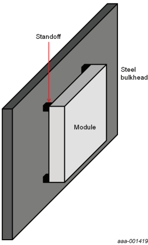
Fig 34. The module mounted on the bulkhead
